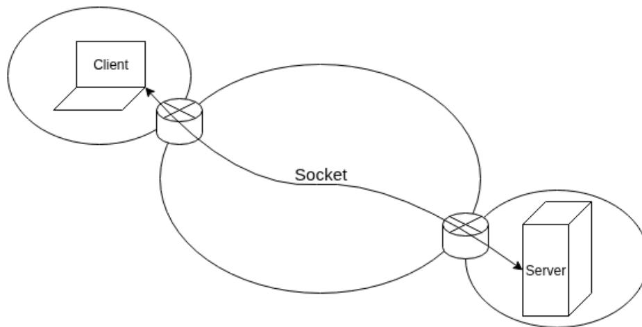
Figura 4.3: Modello client-server
